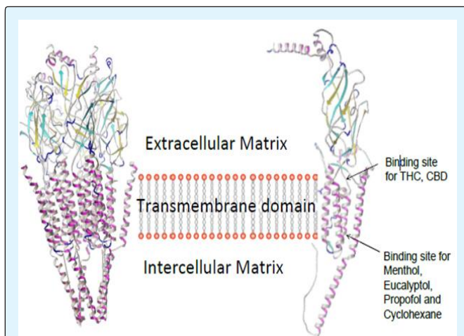
Figure 1: 5-HT 3 chain a receptor.
